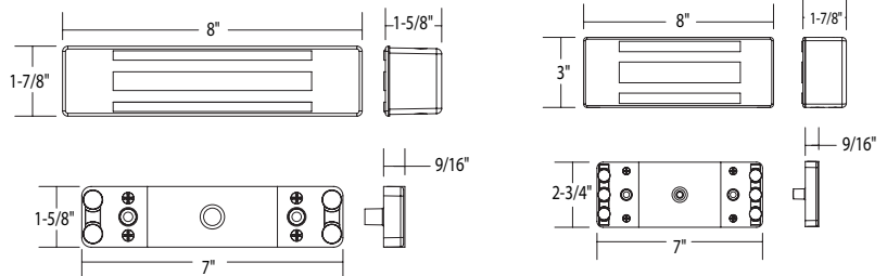
Dimensional Drawing
