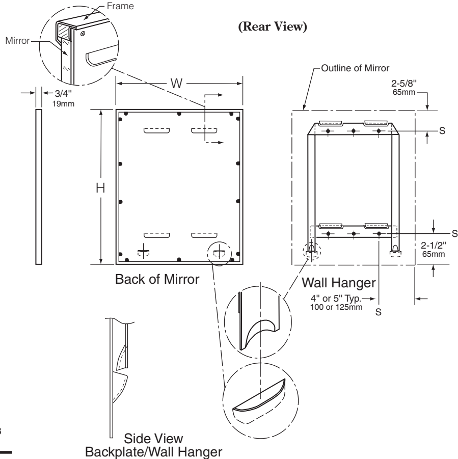
STANDARD SIZE B-280 and B-2808 SERIES MIRRORS
